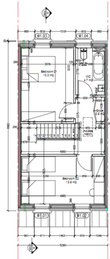
First Floor Plan 1:50 @ A1
