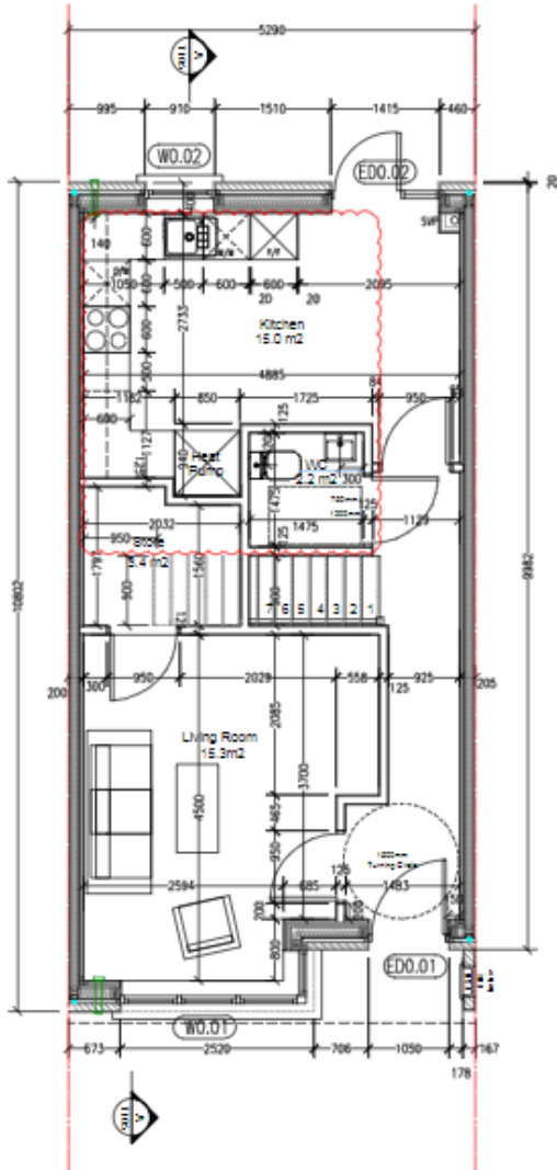
Ground Floor Plan 1:50 @ A1
